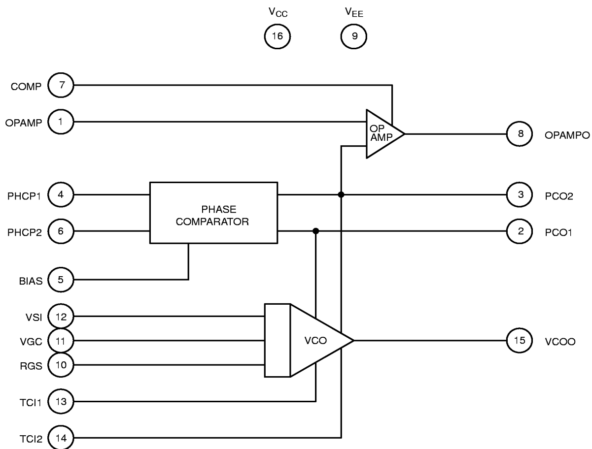
Figure 1. XR-215 Block Diagram
