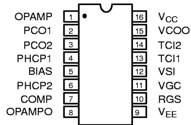
16 Pin PDIP
