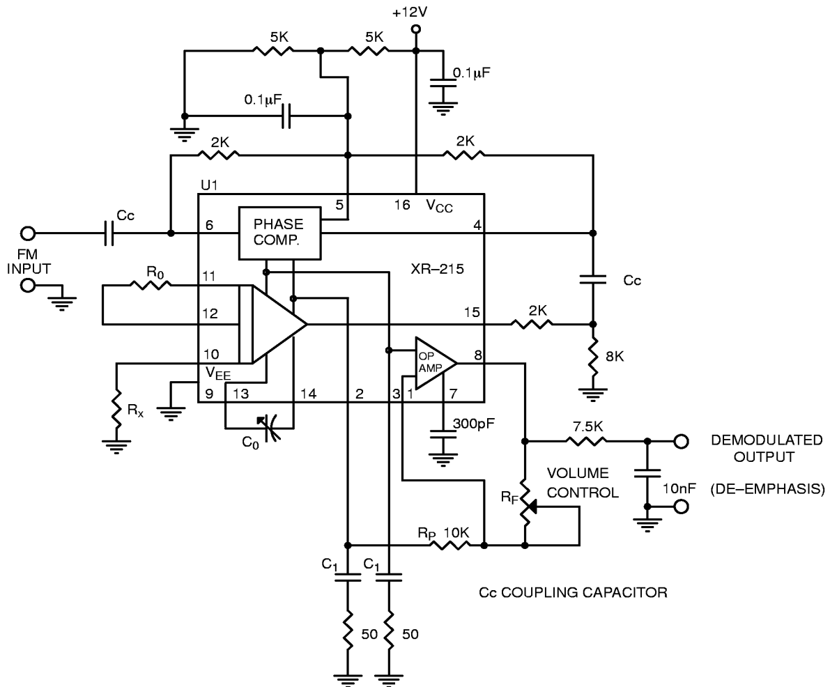
Figure 16. Circuit Connection for FM Demodulation
