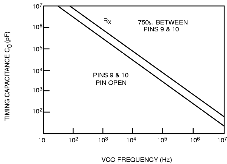
Figure 8. VCO Free Running Frequency vs. Timing Capacitor
