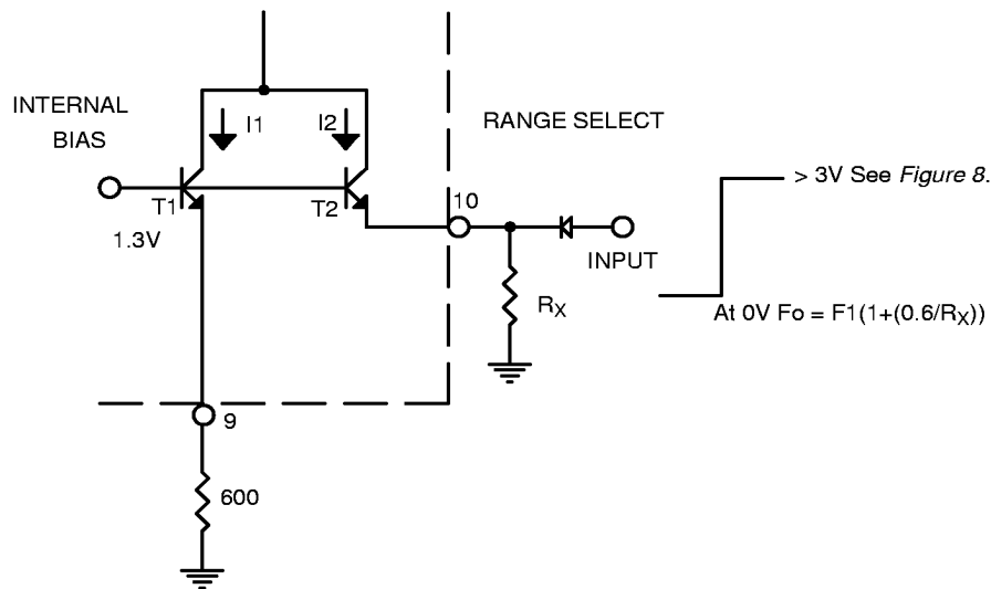
Figure 12. Explanation of VCO Range-Select Controls
