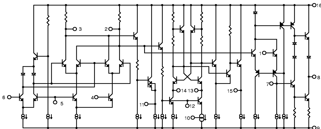
Figure 2. Equivalent Schematic Diagram
