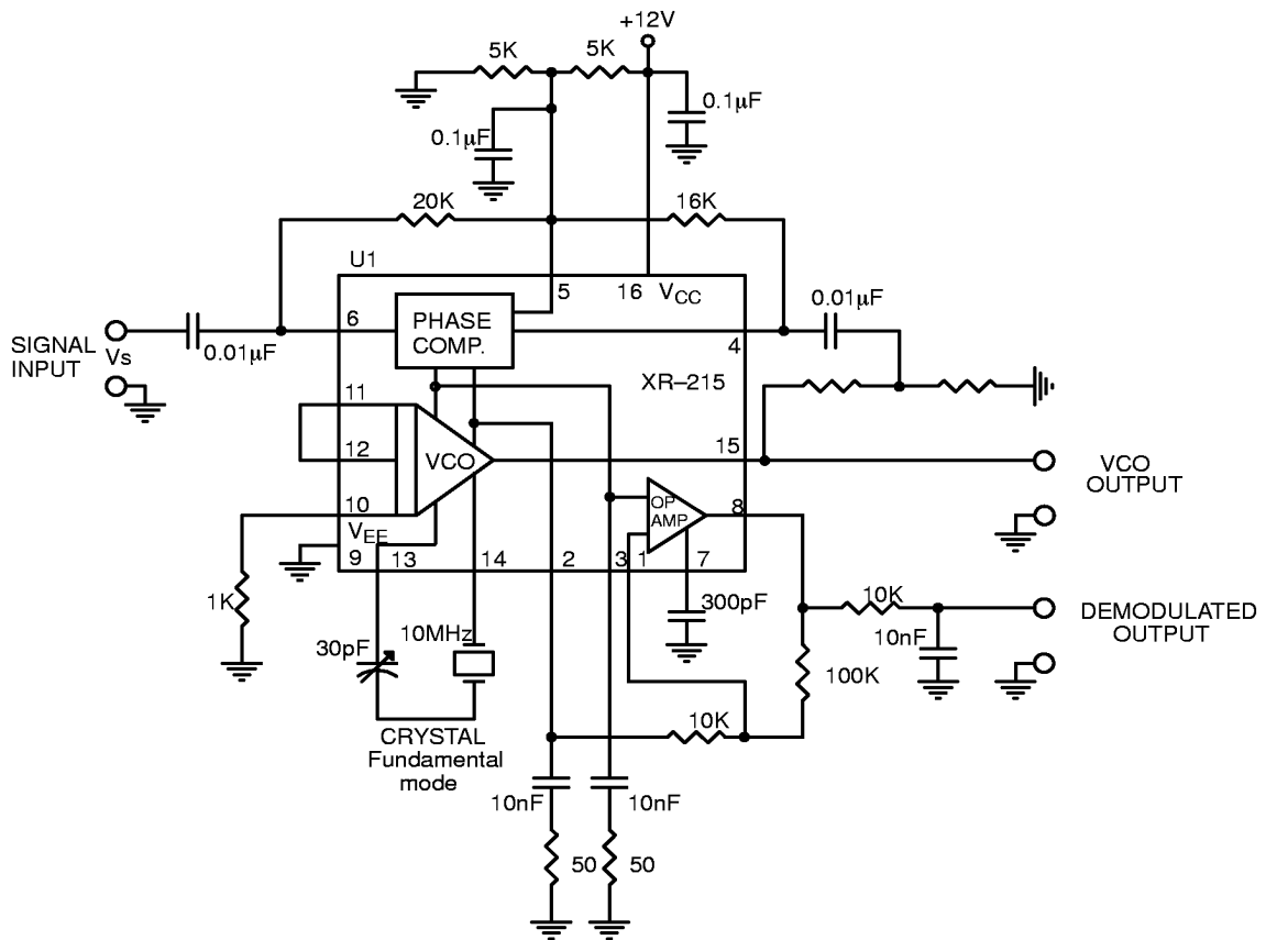
Figure 28. Typical Circuit Connection for Crystal-Controlled Clock Recovery.
