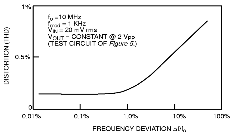
Figure 18. Output Distortion as a Function of FM Deviation
