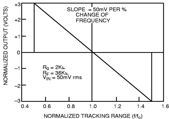
Figure 27. Typical Discriminator Output Characteristics for Tracking Filter Applications
