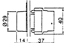
XB2-BV6 ● ZB2-BV0 ●(1) ZB2-BV6 (2)
