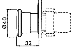
ZB2-BS54 (1)
