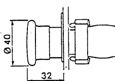
XB2-BC●● ZB2-BC● and 8T - ●(1)
