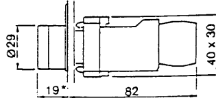
XB2-BW3 (with transformer) ZB2-8W1 ● 8W3 ●, ZB2-BK ● ● ● (1) ZB2-8W03 ● 8W04 ● 8W093 ● (2)
