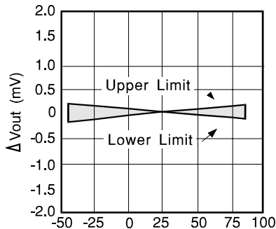
Temperature ^{\circ}\text{C} VRE304J
