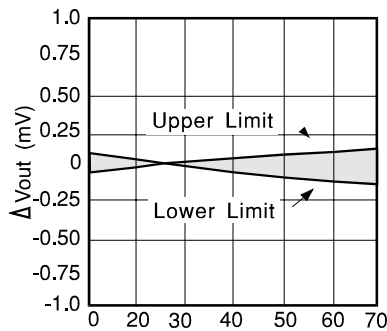
Temperature ^{\circ}\text{C} VRE304A
