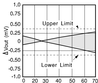
Temperature ^{\circ}\text{C} VRE304B
