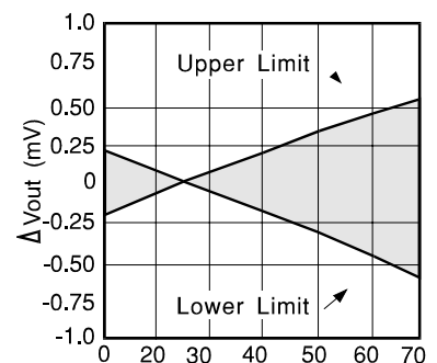
Temperature ^{\circ}\text{C} VRE304C
