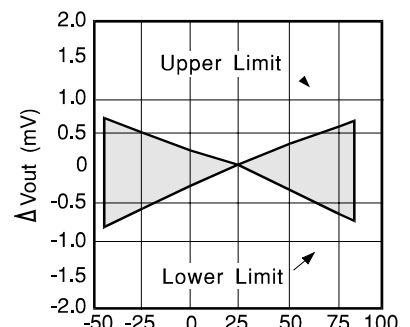
Temperature ^{\circ}\text{C} VRE304L
