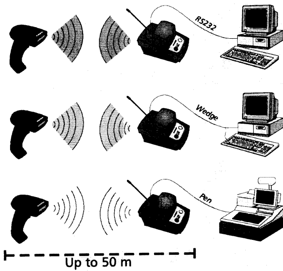
Fig. 1 - DLL6010-R point-to-point connection
