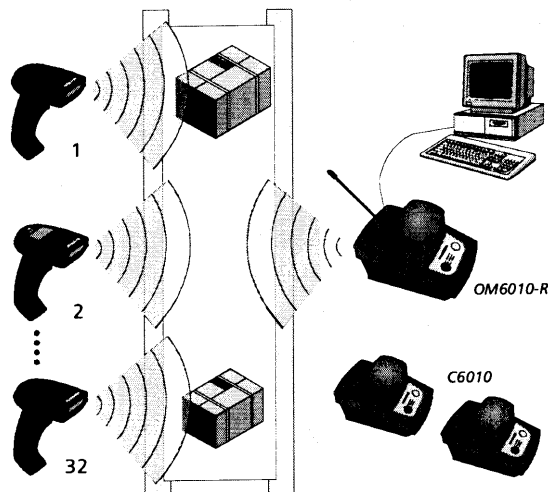
Fig. 2 - DLL6010-R multi-point connection
