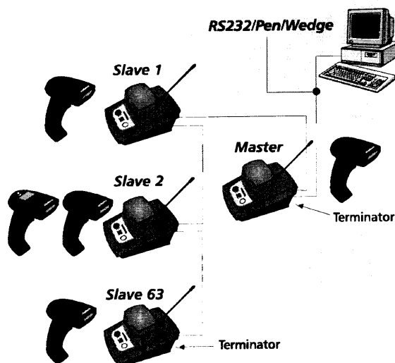
Fig. 3 - DLL6010-R network (Echelon kit required)
