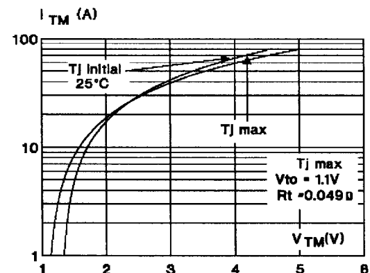
Fig. 5 :On-state characteristics (maximum values).
