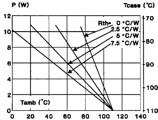
Fig. 3 :Correlation between maximum mean power dissipation and maximum allowable temperatures ( T_{amb} and T_{case} ) for different thermal resistances heatsink + contact (AVS10CB).
