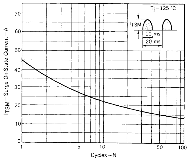
Fig. 2 I_{TSM} RATING
