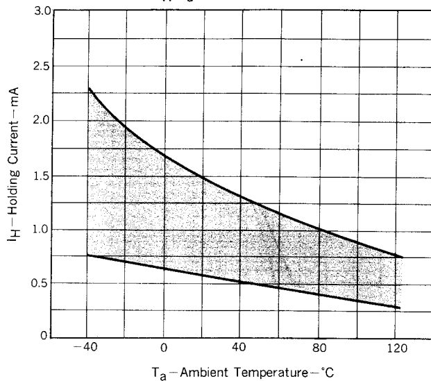
Fig. 8 I_H-T_a TYPICAL DISTRIBUTION
