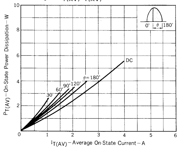
Fig. 9 P_T(AV) \cdot I_T(AV) CHARACTERISTIC
