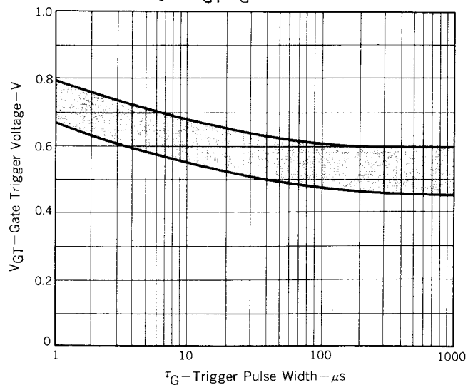
Fig. 7 v_{GT}-\tau_G DISTRIBUTION
