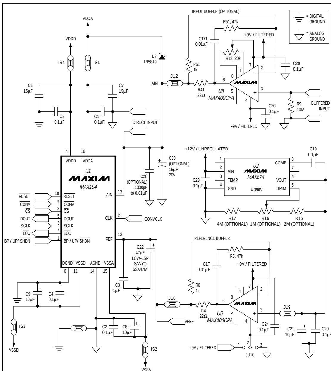
Figure 1. MAX194 EV Kit Schematic
