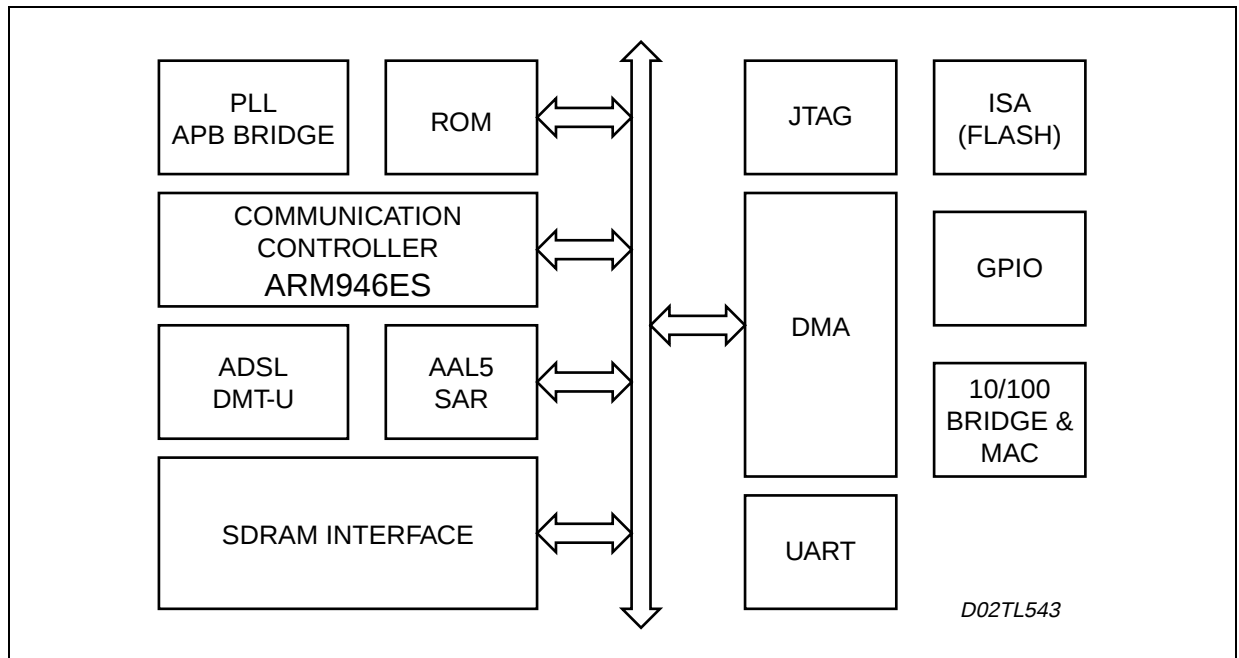
Figure 2. Block diagram
