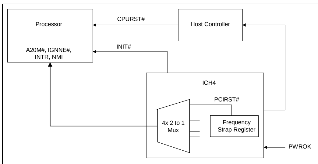
Figure 5-13. Signal Strapping
