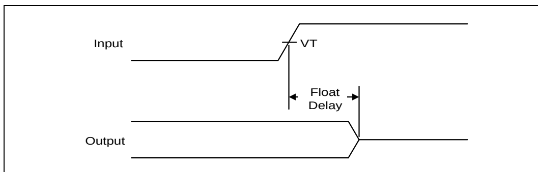
Figure 17-5. Pulse Width
