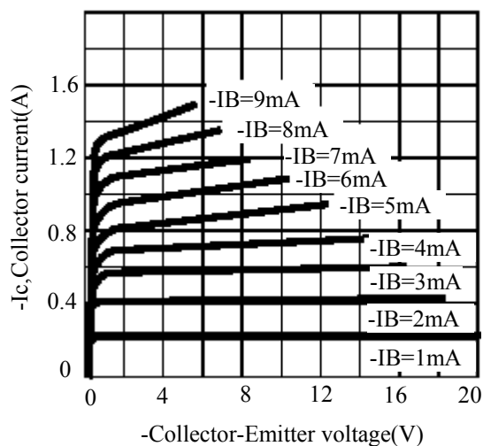
Fig.1 Static characteristics
