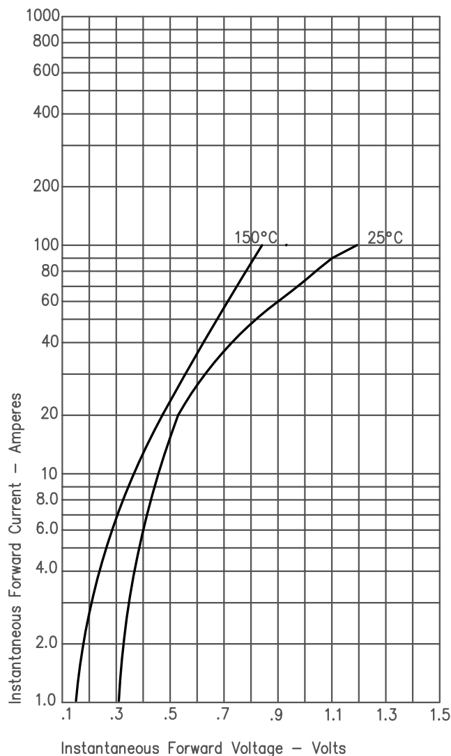
Figure 1 Typical Forward Characteristic — Per Leg
