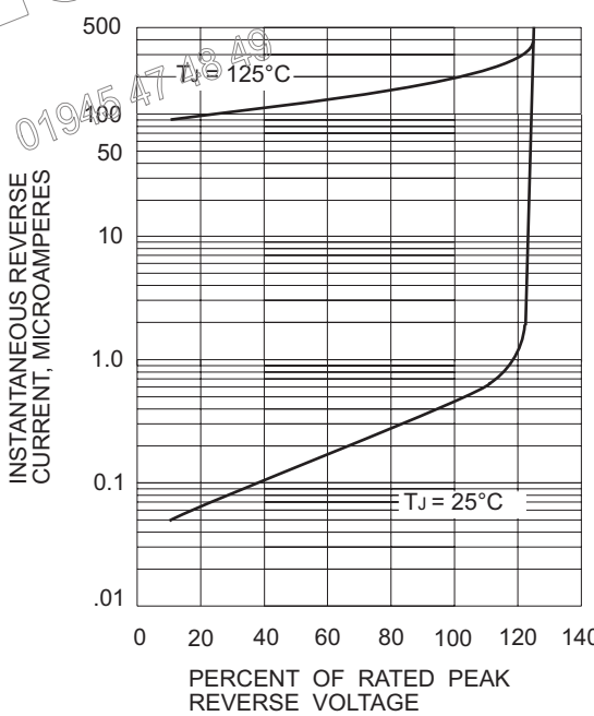
FIG 4 : TYPICAL REVERSE CHARACTERISTICS PER ELEMENT
