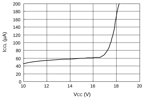
Latch mode supply current ( I_{CCL} ) vs. supply voltage ( V_{CC} ) Enlarged
