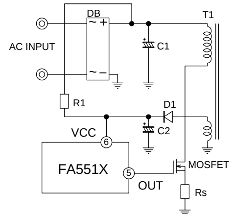
Fig. 19 Startup circuit (2)
