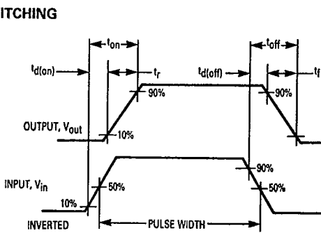
Figure 14. Switching Waveforms
