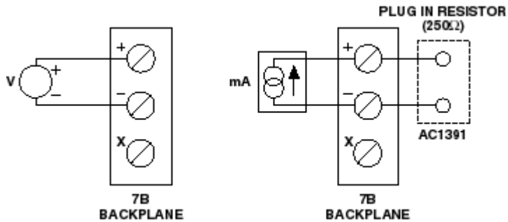
Figure 3 7B33 Input Field Connections
