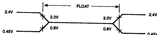
Figure 7. Float Waveform
