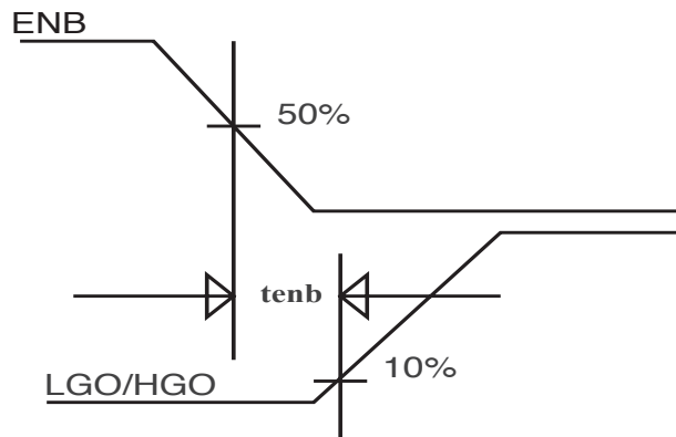
Figure 4. ENABLE Waveform Definitions
