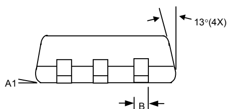
SOT 223 (T6) Package
