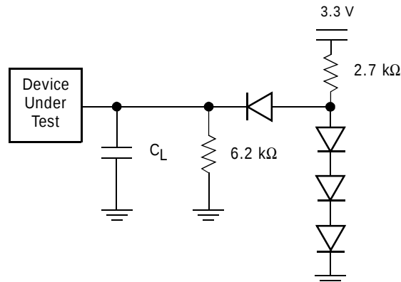
Figure II. Test Setup
