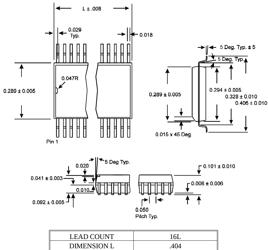
Figure 5: 16-Pin SOIC Package
