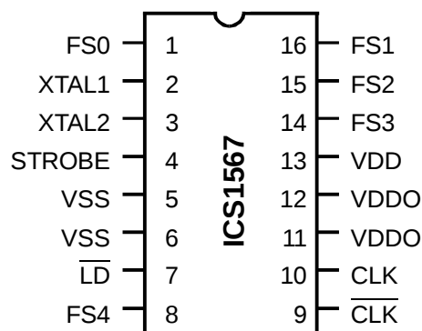
16-Pin SOIC
