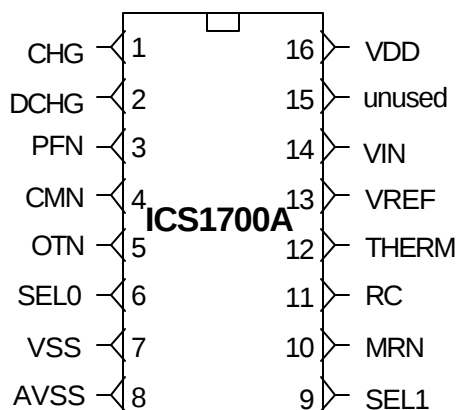
16-Pin DIP
