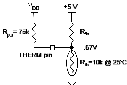
Figure 8: Voltage divider at the THERM pin at 25^\circ\text{C}
