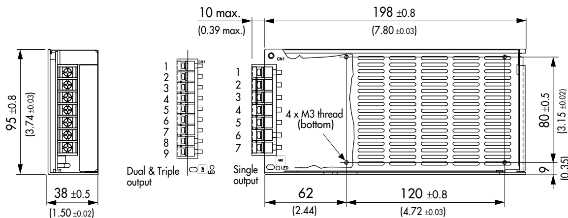
Pin-Out
