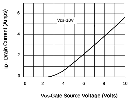
Transfer Characteristics
