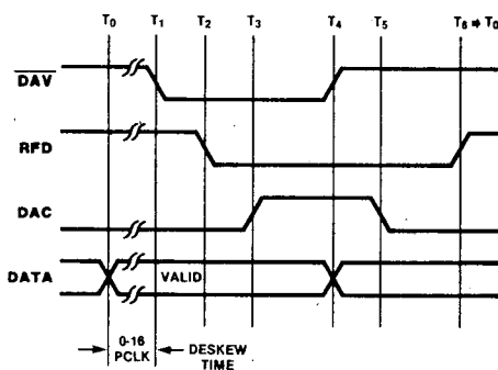
Figure 3-13. 3-Wire Output Handshake Timing Diagram
