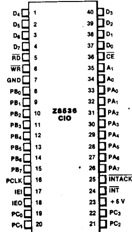
Figure 2. Pin Assignments
