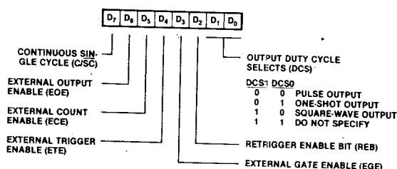
Figure 2-15. Counter/Timer Mode Specification Registers
