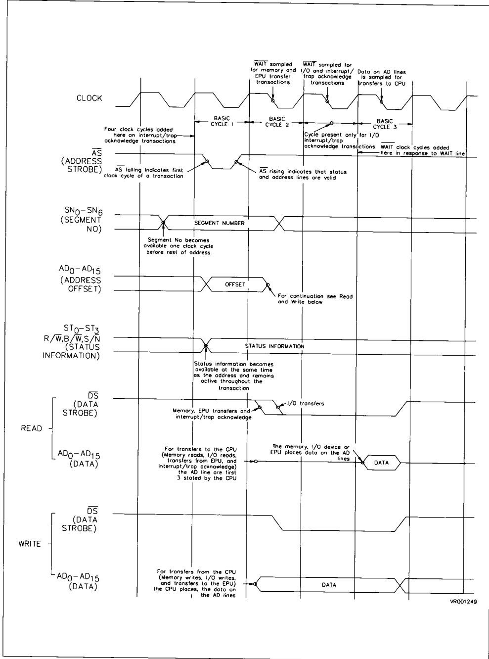
Figure 2-5. Transaction Timing
