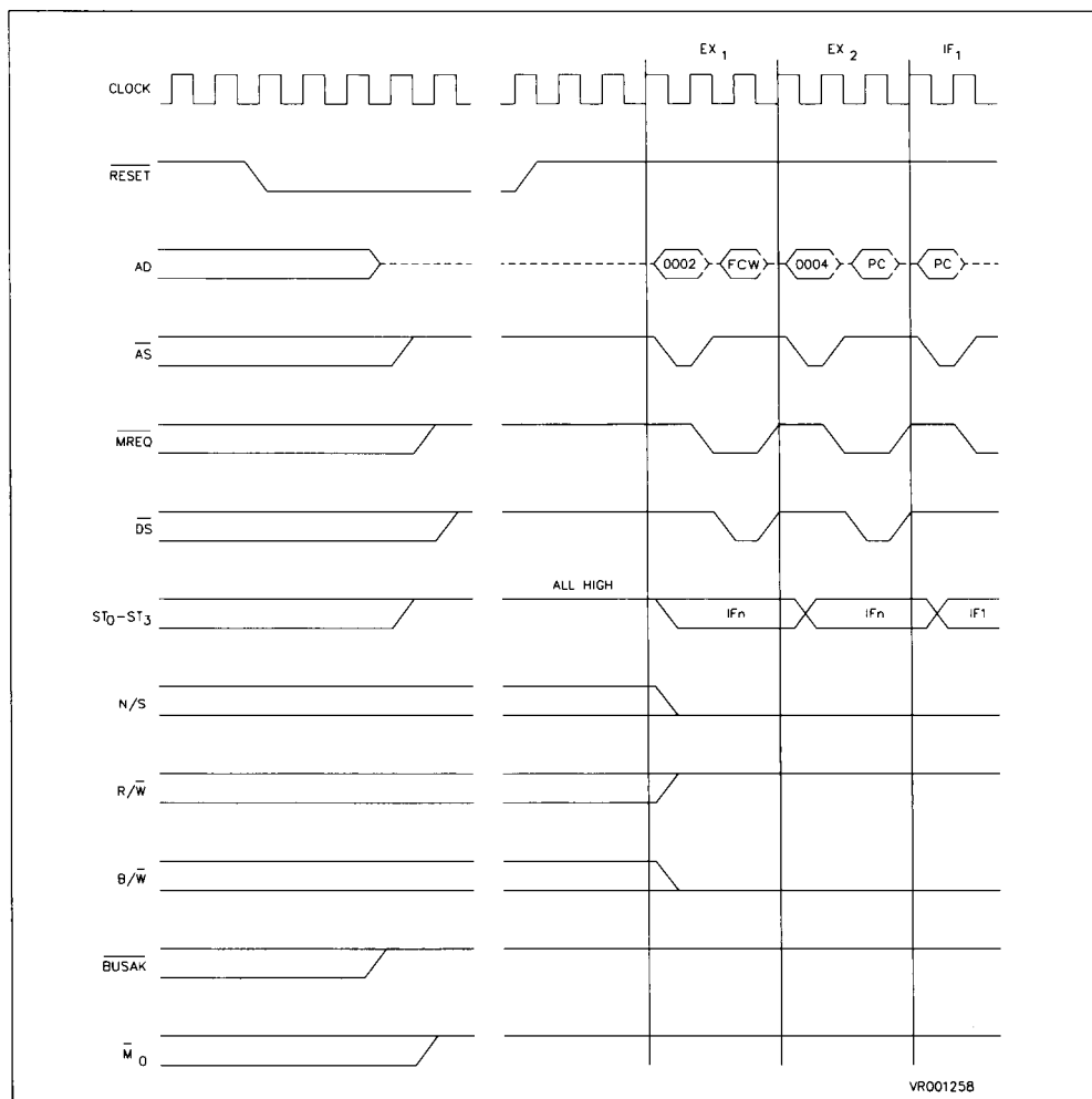
Figure 2-14. Reset Timing
