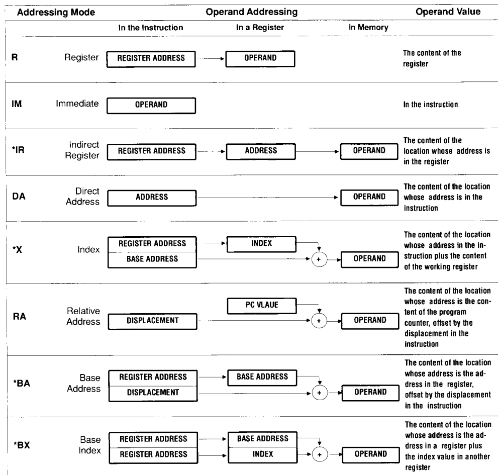
Figure 6-1. Addressing Modes
