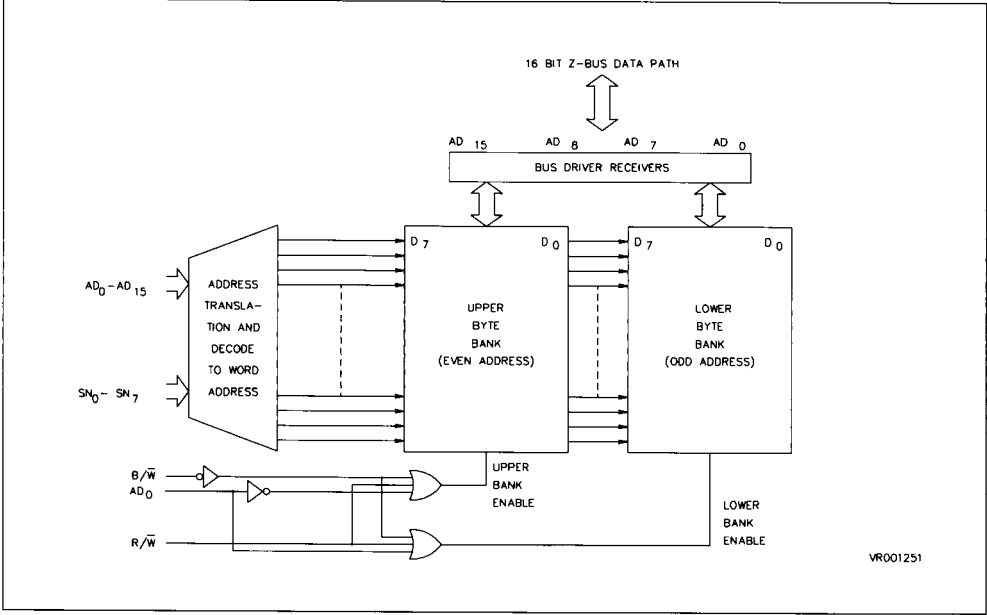
Figure 2-7. Memory Organization
