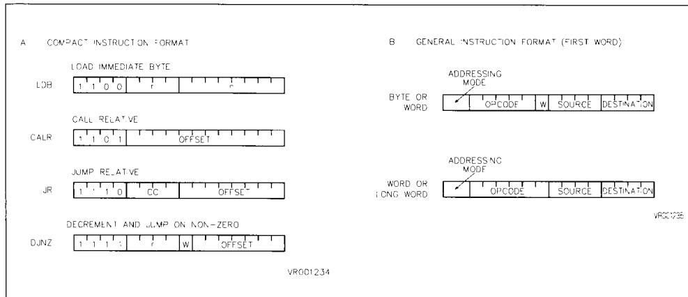
Figure 3-7. Instruction Formats
