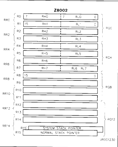
Figure 1-3b. Z8002 General-Purpose Registers
