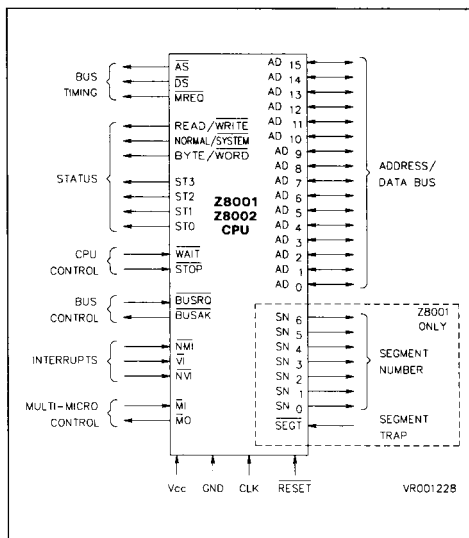
Figure 1-1. Logic Function
