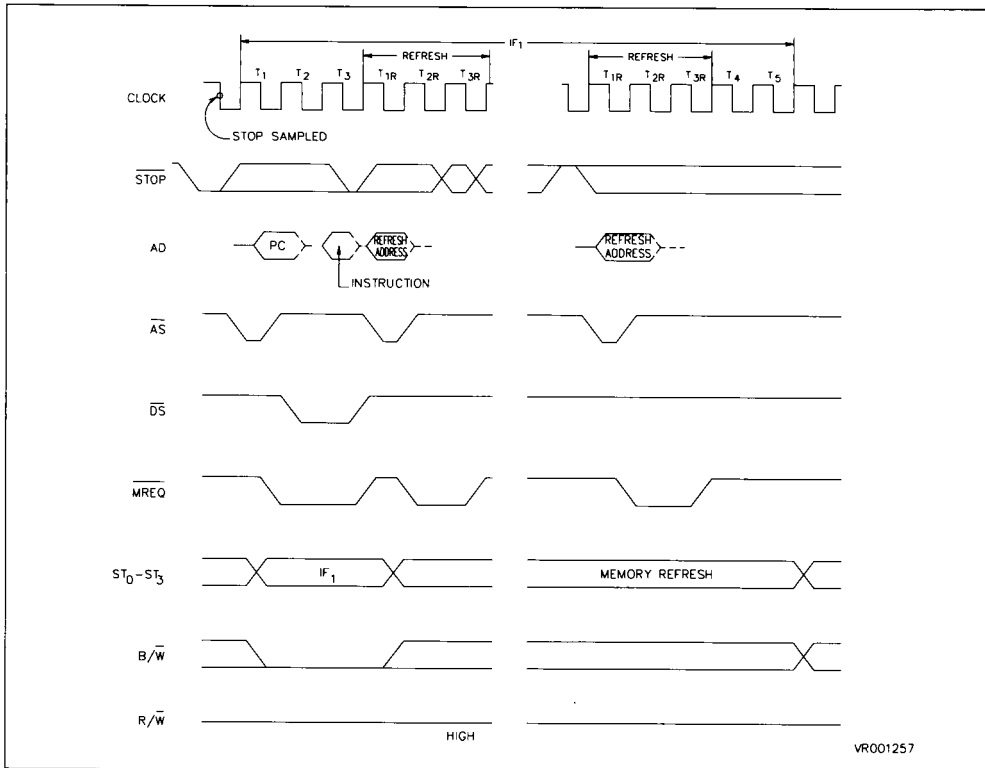
Figure 2-13. Stop Timing
