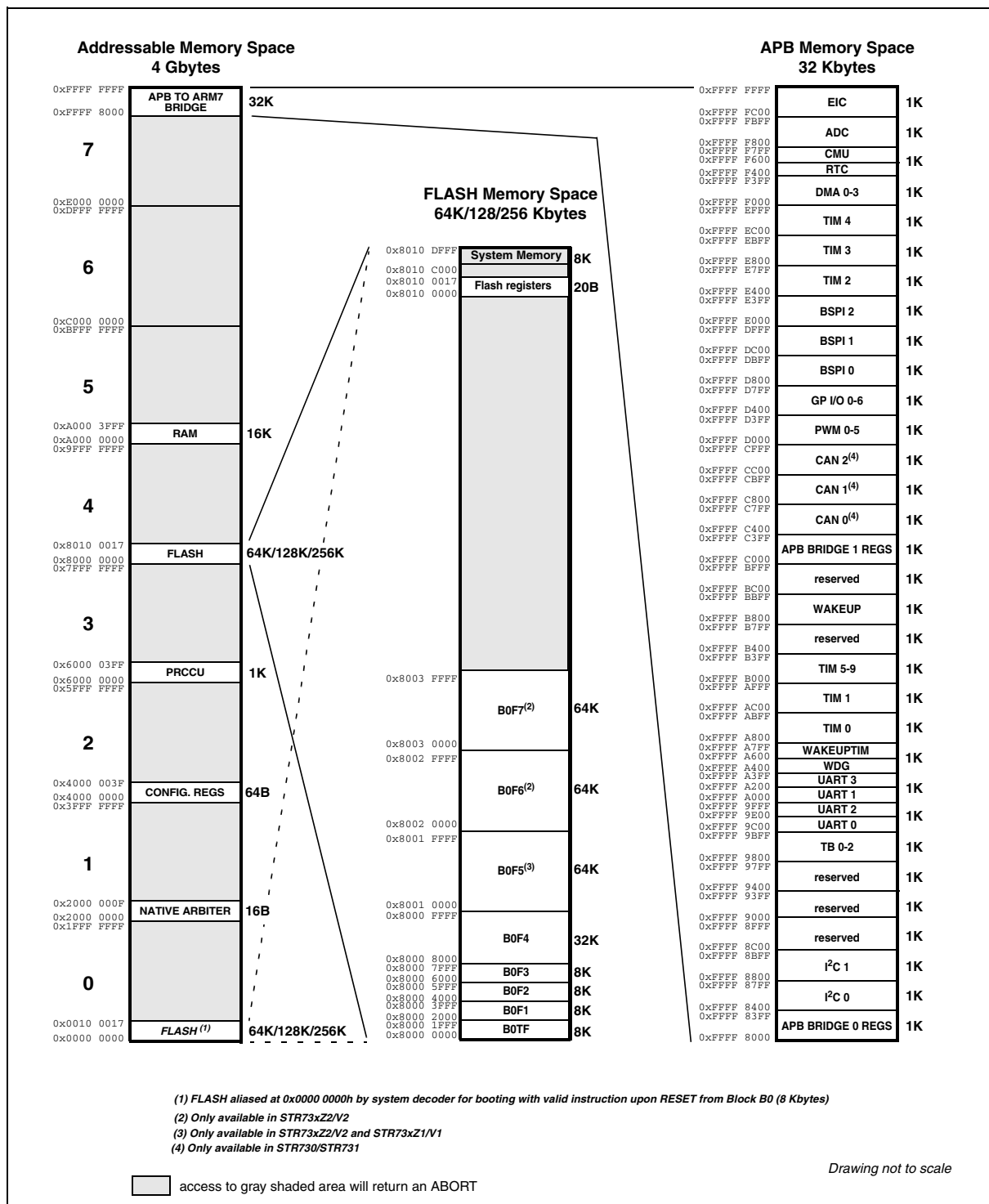
Figure 5. Memory Map
