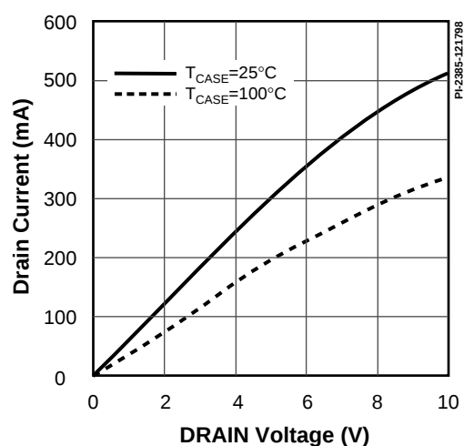
OUTPUT CHARACTERISTIC
