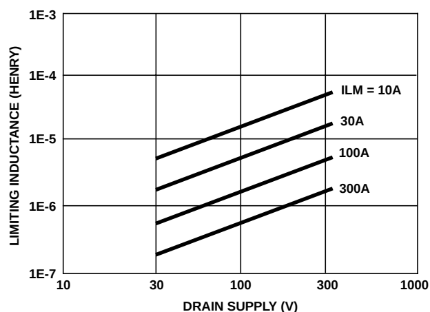
FIGURE 2. TYPICAL DRAIN INDUCTANCE REQUIRED TO LIMIT GAMMA DOT CURRENT TO I_{AS}
