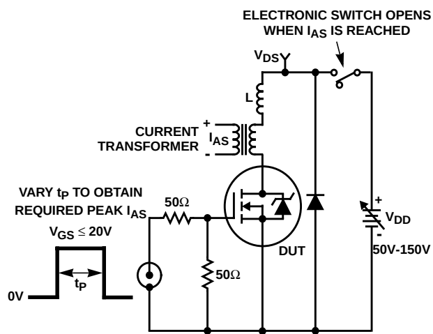
FIGURE 9. UNCLAMPED ENERGY TEST CIRCUIT
