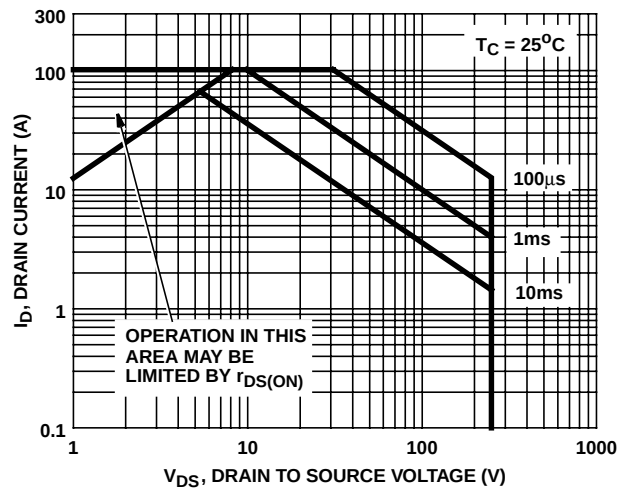
FIGURE 4. FORWARD BIAS SAFE OPERATING CURVE
