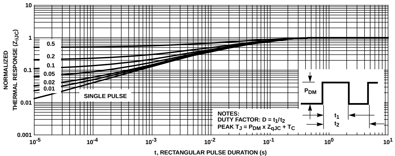
FIGURE 7. NORMALIZED MAXIMUM TRANSIENT THERMAL RESPONSE
