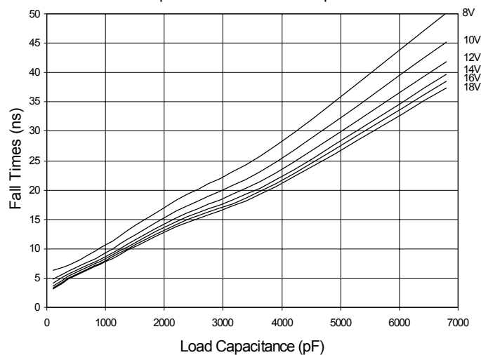
Fig. 7 Output Fall Times vs. Load Capacitance
