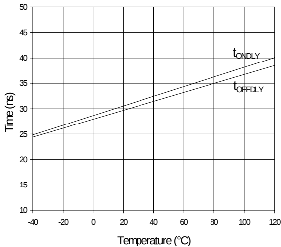
Fig. 19 Propagation Delay vs. Case Temperature C_L = 2500\text{pF} , V_{CC} = 18\text{V}
