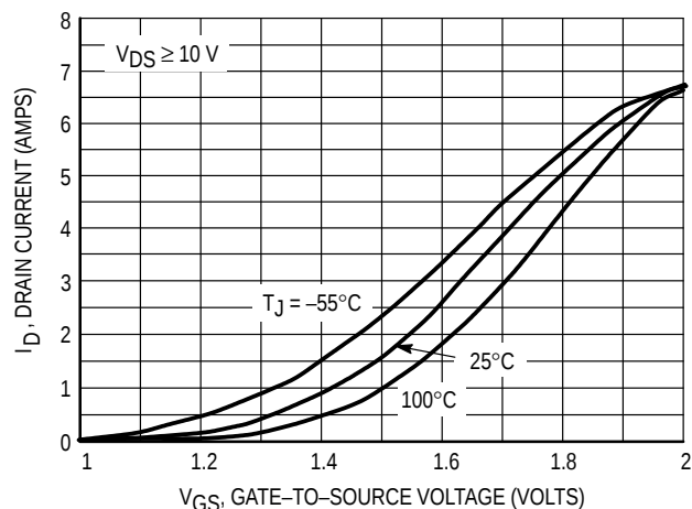
Figure 4. Transfer Characteristics
