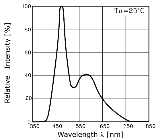
Fig. 4 Spectrum Distribution
