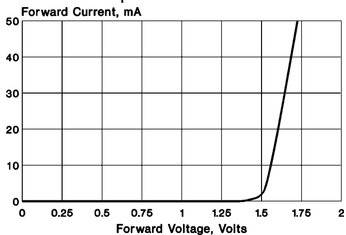
Input Characteristics
