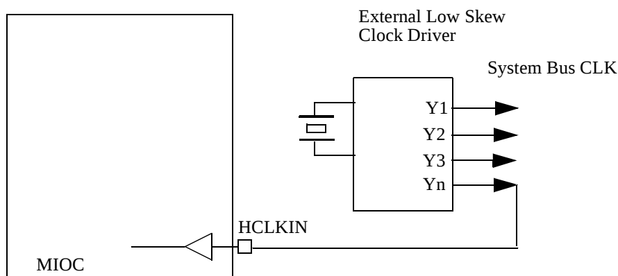
Figure 11-1: Host Clock Generation and Distribution
