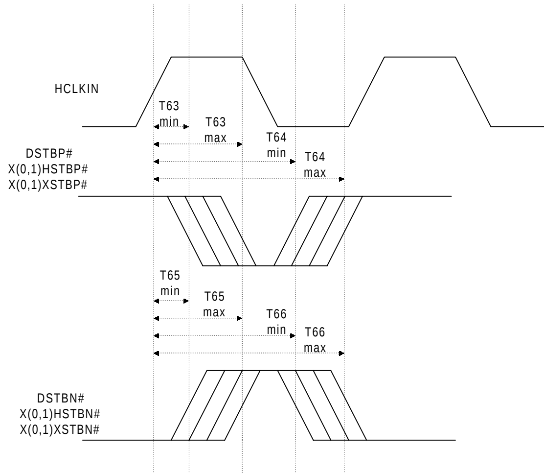
Figure 12-7: Source Synchronous Strobe Timing
