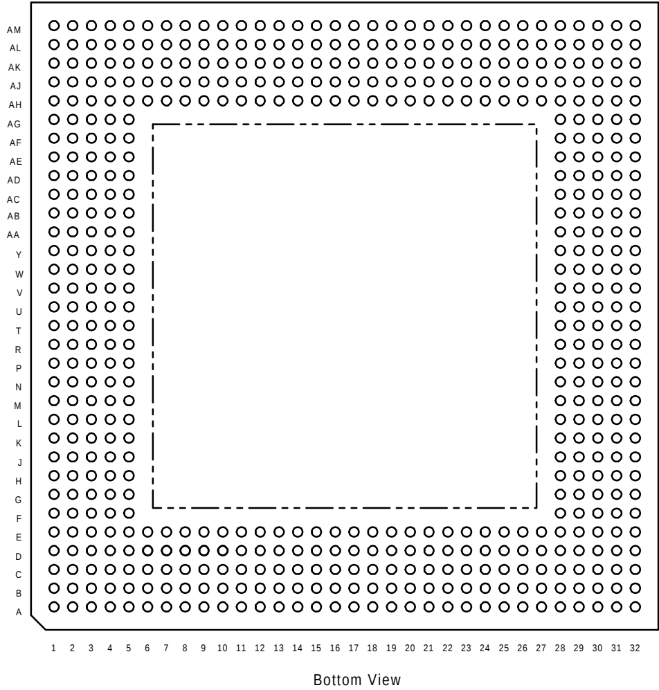
Figure 12-17: 540 PBGA Pin Grid
