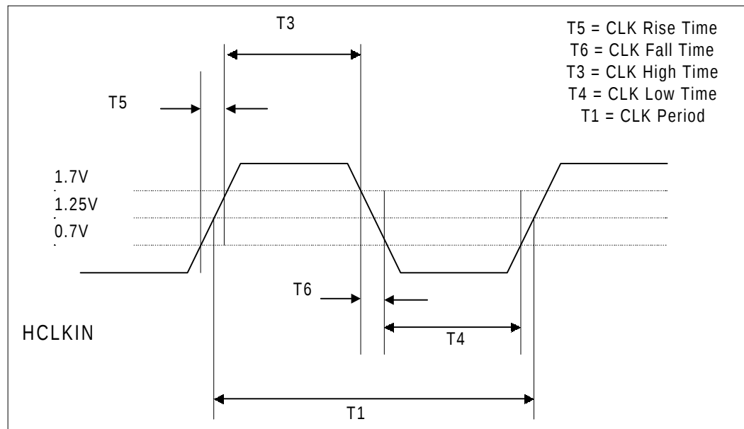
Figure 12-6: CLK Waveform
