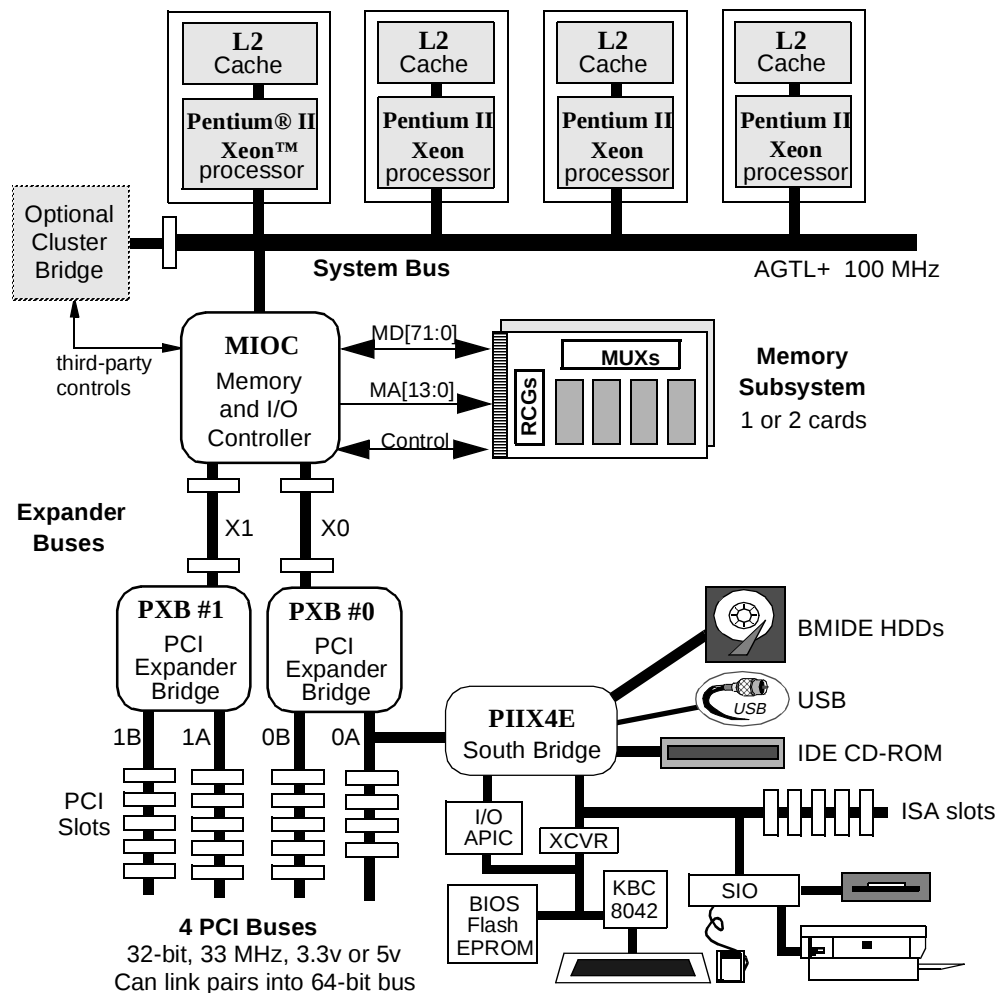
Figure 1-1: Simplified Intel® 450NX PCIsset System Block Diagram
