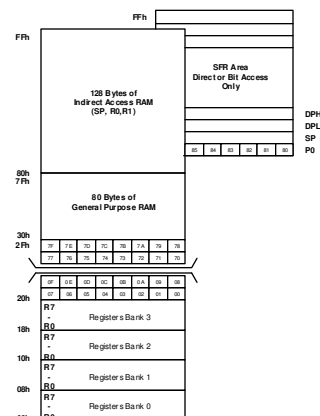
FIGURE 5: VRS550 / VRS560 RAM STRUCTURE
