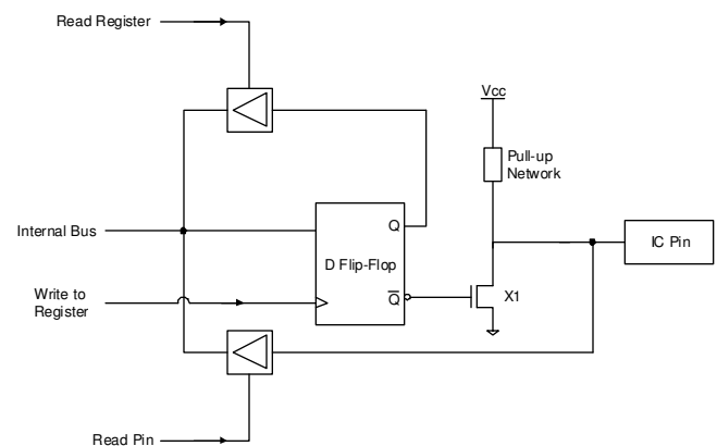
FIGURE 7: GENERAL STRUCTURE OF THE OUTPUT STAGE OF P1, P2 AND P3
