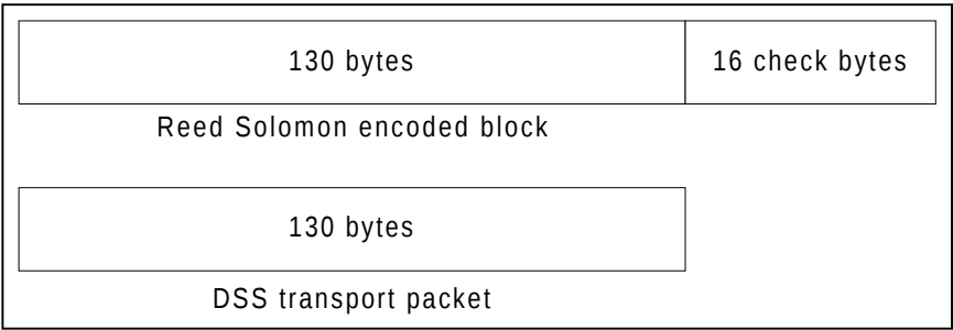
Figure 8. DSS block structure.
