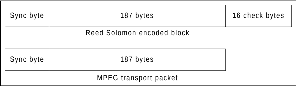
Figure 7. DVB block structure.
