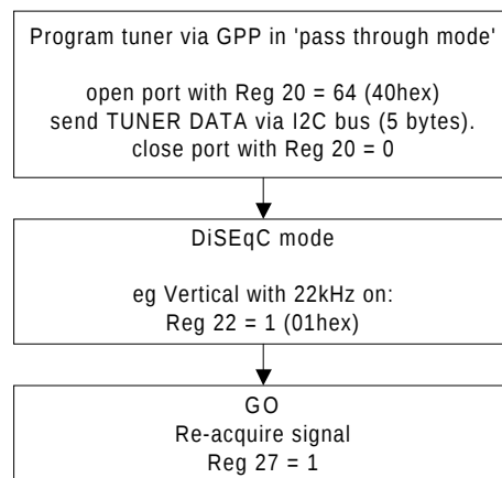
Figure 14. Simple channel change sequence.
