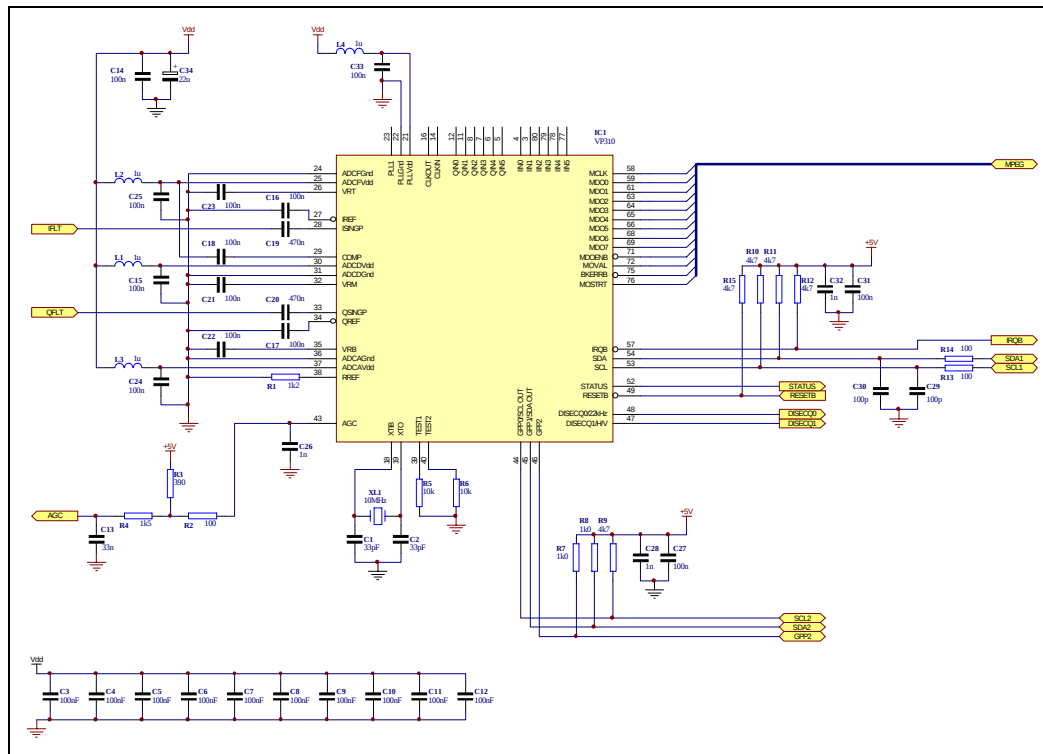
Figure 20. Application Schematic.
