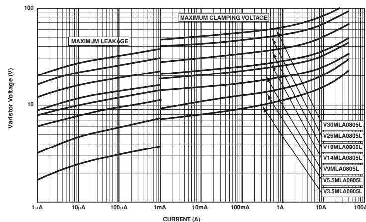
FIGURE 6. LIMIT V-I CHARACTERISTIC FOR V3.5MLA0805L TO V30MLA0805L
