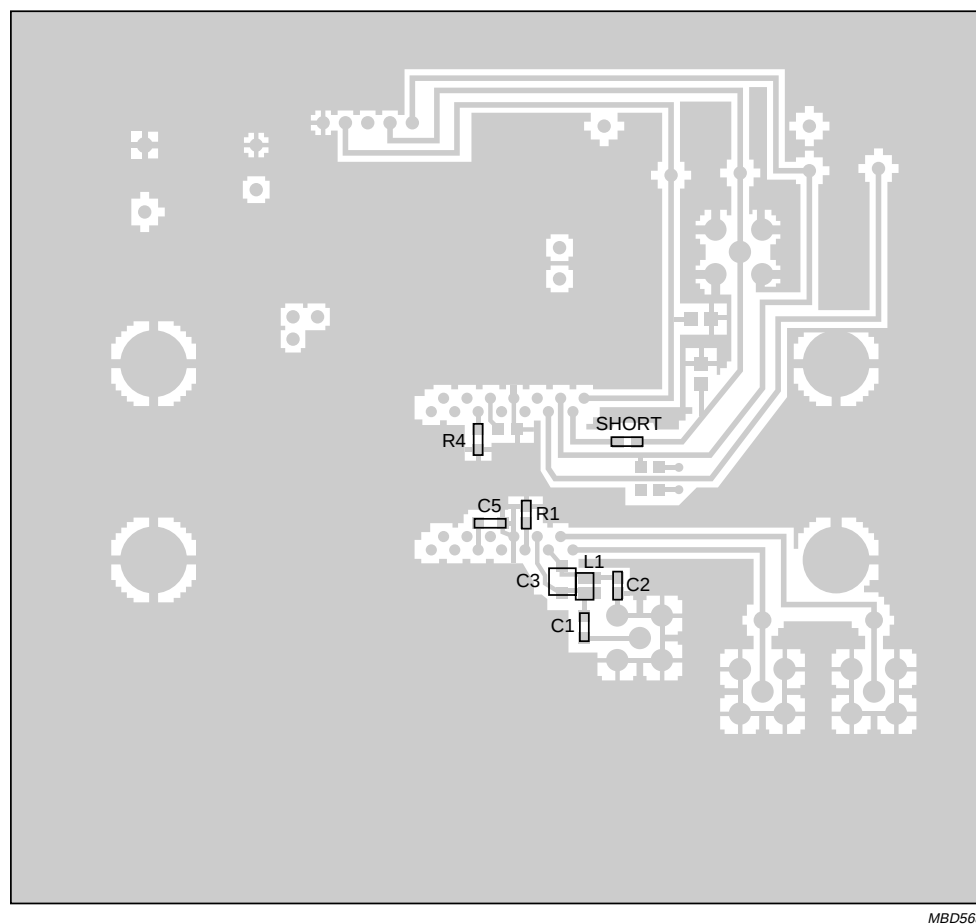
Fig.21 PCB bottom view with components for SO28; test circuit Fig.4.
