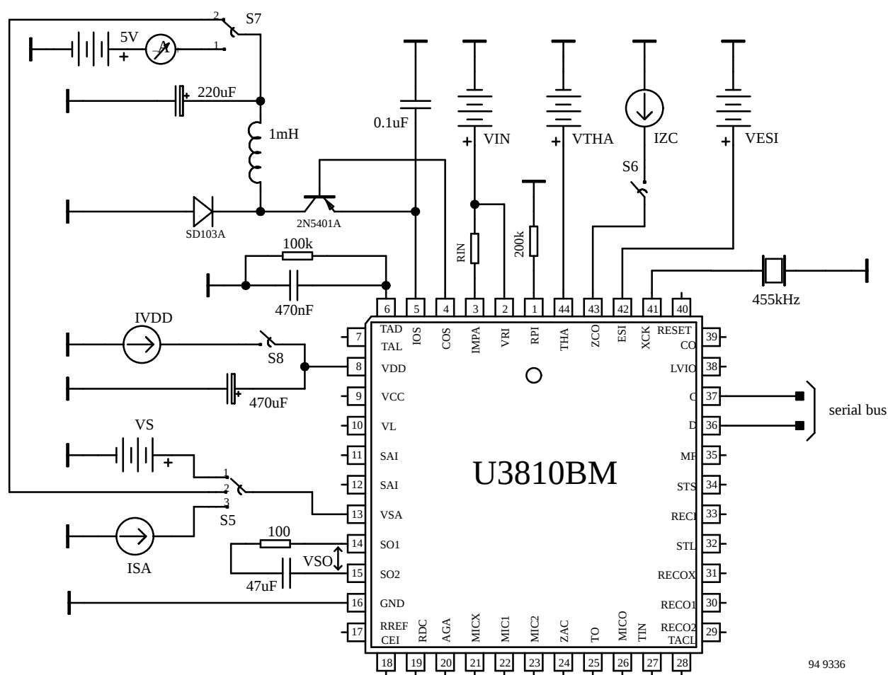
Figure 10 Test circuit
