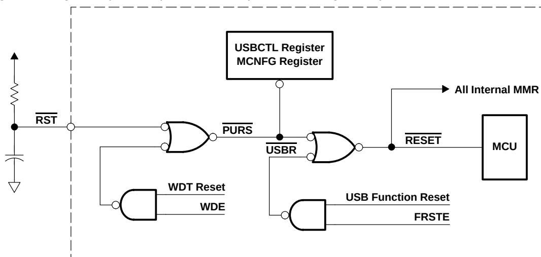
Figure 2–2. Reset Diagram
