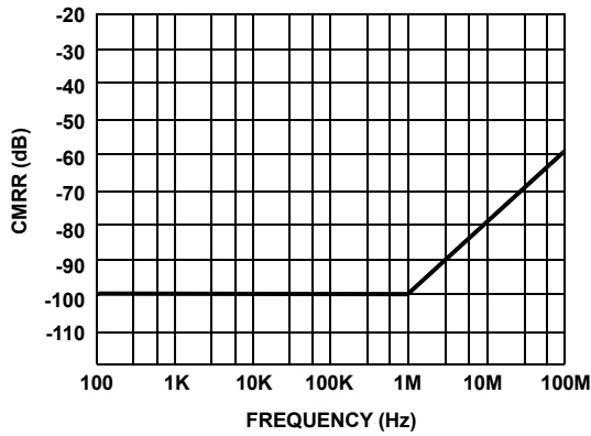
FIGURE 23. CMRR
