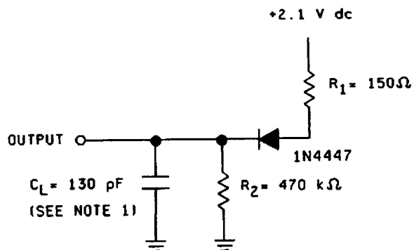
OUTPUT LOAD CIRCUIT FOR \overline{DTACK}
