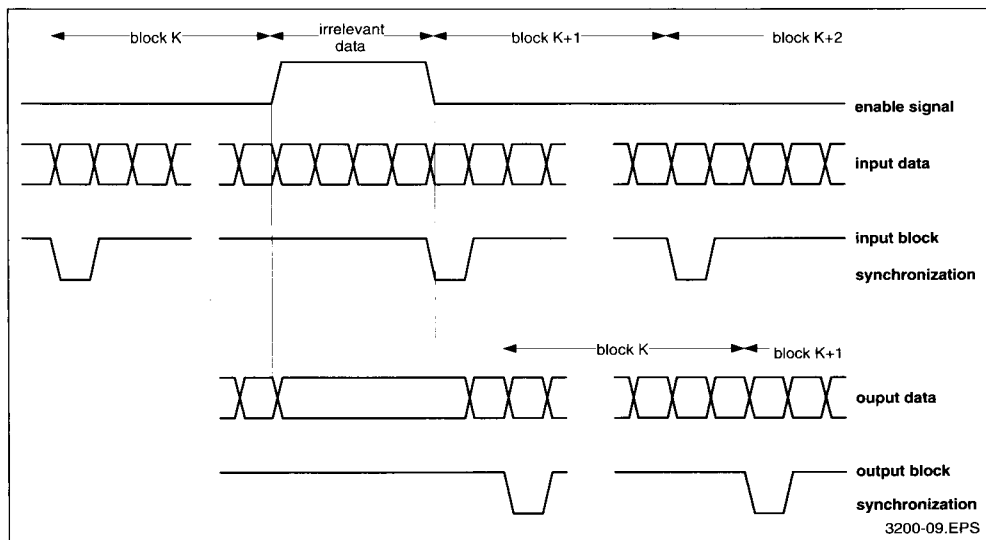
Figure 8 : Burst Block Flow
