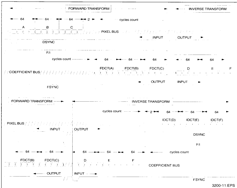
Figure 9 : Mixed 8x8 FDCT/IDCT Example Waveforms
