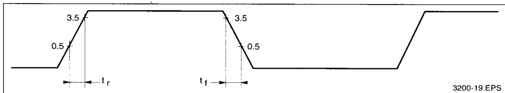
Output Timing Diagram
