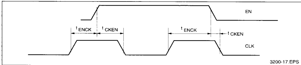
Clock Timing Diagram
