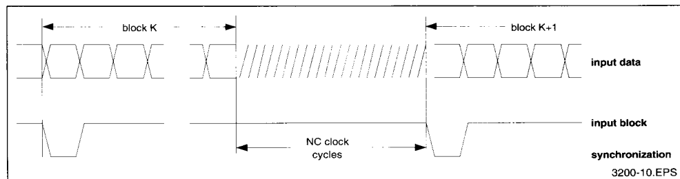
Figure 8 : Burst Block Flow
