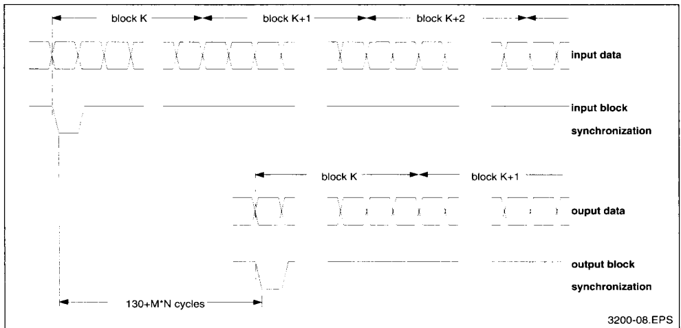
Figure 6 : Continuous Block Flow-2
