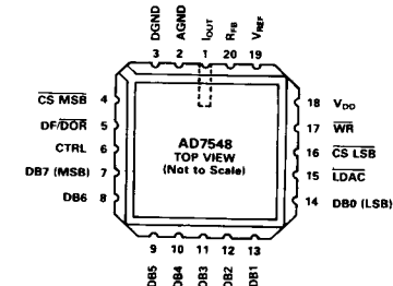
E Package
