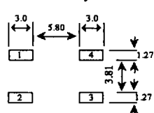
Recommended Solder Pad Layout
