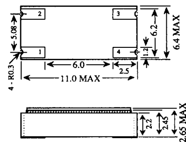
Pin Connections #1 E/D #3 Output #2 GND #4 +5 VDC
