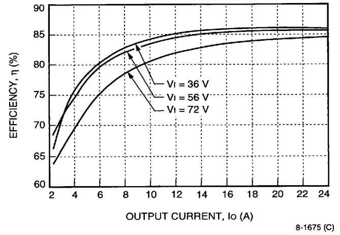
Figure 4. Typical FW150S6R5 Efficiency vs. Output Current at Room Temperature 8-1675 (C)
