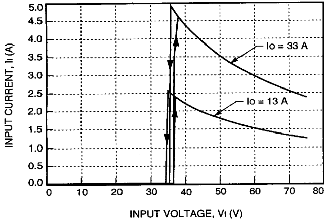
Figure 1. Typical FW150S6R5 Input Characteristics at Room Temperature 8-1672 (C)
