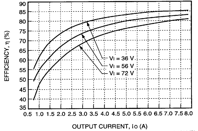
Figure 3. Typical FW050S6R5 Efficiency vs. Output Current at Room Temperature 8-1674 (C)
