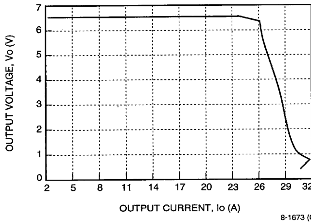
Figure 2. Typical FW150S6R5 Output Characteristics at Room Temperature and 48 V Input 8-1673 (C)
