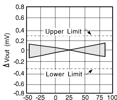
Temperature ^{\circ}\text{C} VRE302-6K
