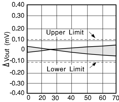
Temperature ^{\circ}\text{C} VRE302-6A
