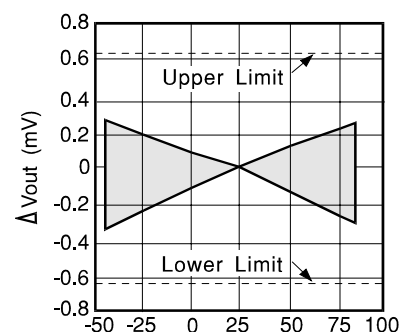
Temperature ^{\circ}\text{C} VRE302-6L
