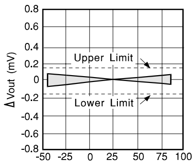
Temperature ^{\circ}\text{C} VRE302-6J
