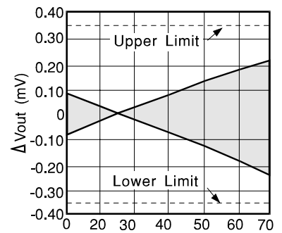
Temperature ^{\circ}\text{C} VRE302-6C
