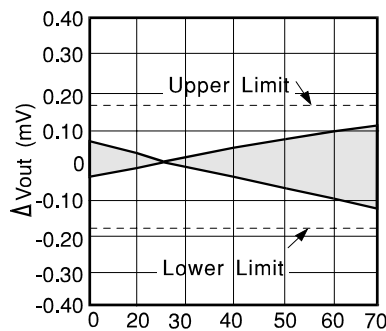
Temperature ^{\circ}\text{C} VRE302-6B
