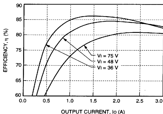
Figure 22. LW015A Typical Efficiency vs. Output Current at T_c = 25\text{ }^{\circ}\text{C}
