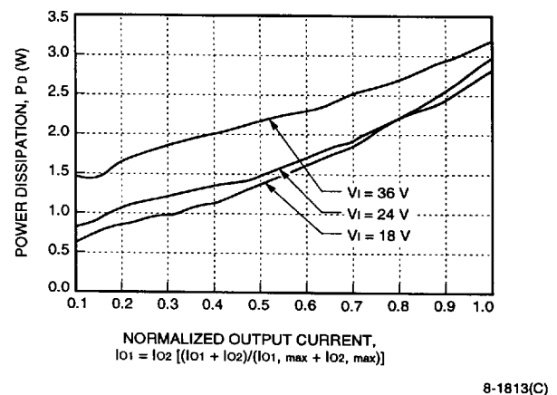
Figure 52. LC010AJ, BK, CL Typical Power Dissipation vs. Normalized Output Current at T_c = 25^\circ\text{C}
