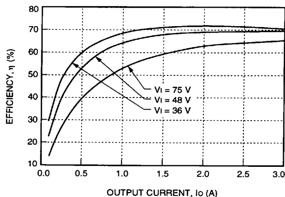
Figure 24. LW010D, 015D Typical Efficiency vs. Output Current at T_c = 25\text{ }^{\circ}\text{C}
