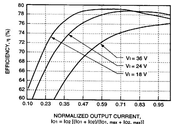
Figure 21. LC010AJ, BK, CL Typical Efficiency vs. Normalized Output Current at T_c = 25^\circ\text{C}
