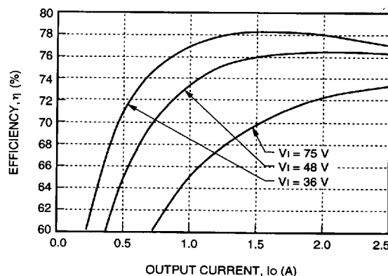
Figure 27. LW010F Typical Efficiency vs. Output Current at T_c = 25\text{ }^{\circ}\text{C}
