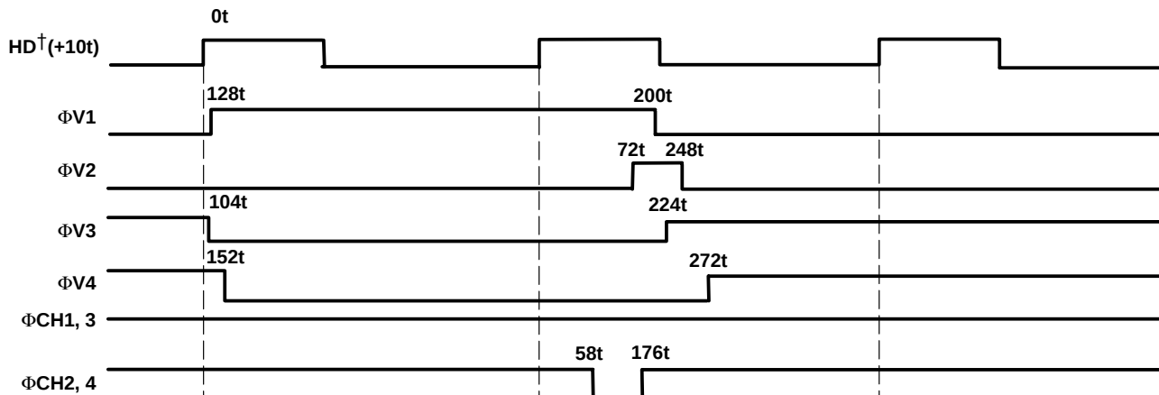
2) V-Rate Readout Detailed Timing Chart: (Frame Mode, Even Field)
